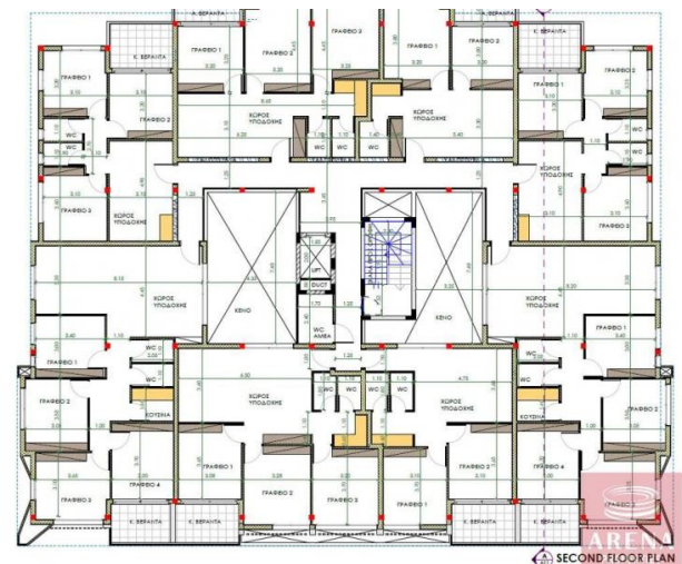
AREE SECOND FLOOR PLAN
