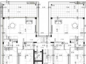
GROUND FLOOR
