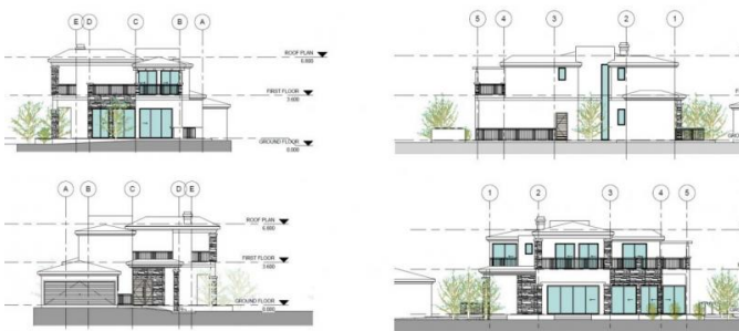
Elevations
