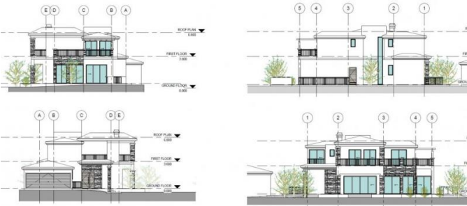
Elevations
