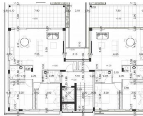
1ST FLOOR
